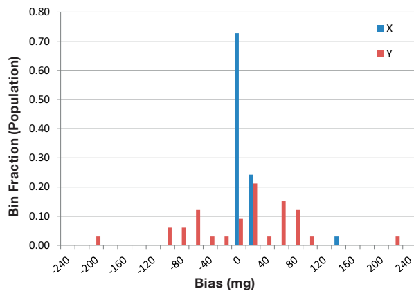
Figure 5.5 CAS215 (96g) Bias Distribution at 20°C
