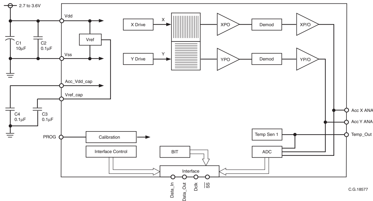
Figure 1.1 CAS200 Functional Block Diagram
