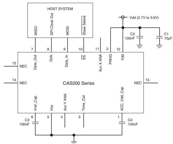
Figure 7.4 Digital Output Setup
