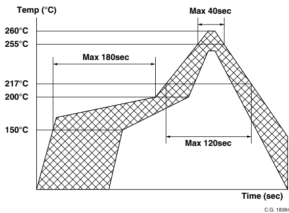
Figure 10.1 Recommended Reflow Solder Profile
