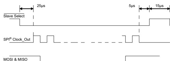
Figure 7.5 SPI® Timing Diagram
