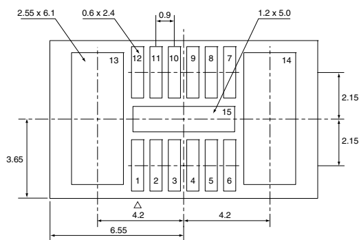
Figure 7.2 Recommended Pad Layout
