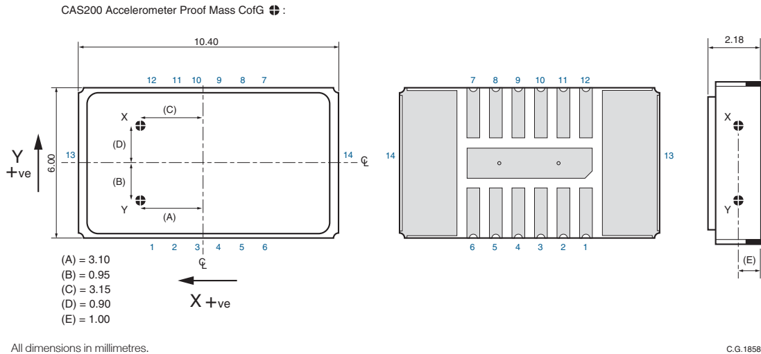
Figure 1.2 CAS200 Overall Dimensions
