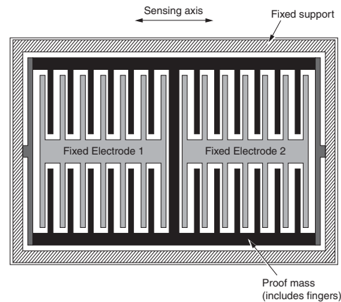
Figure 13.3(a) Schematic of Accelerometer Structure
