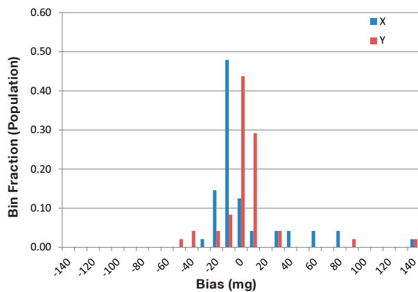
Figure 5.3 CAS213 (10g) Bias Distribution at 20°C
