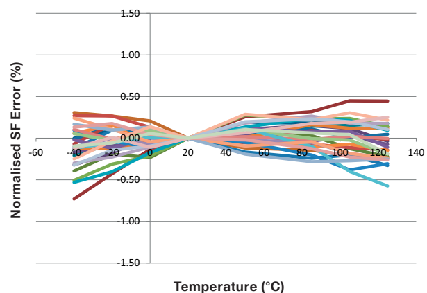
Figure 5.20 CAS215 (96g) Accelerometer Y SF Error with Temperature
