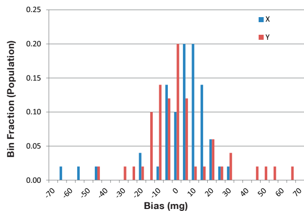
Figure 5.2 CAS212 (2.5g) Bias Distribution at 20°C
