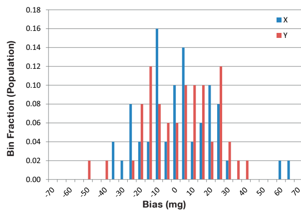
Figure 5.4 CAS214 (30g) Bias Distribution at 20°C
