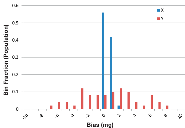
Figure 5.1 CAS211 (0.85g) Bias Distribution at 20°C
