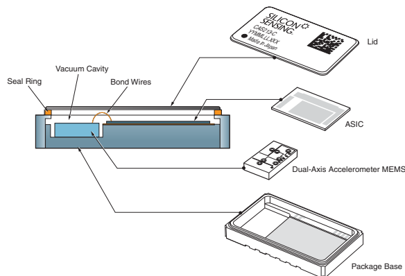
Figure 13.1 CAS200 Main Components
