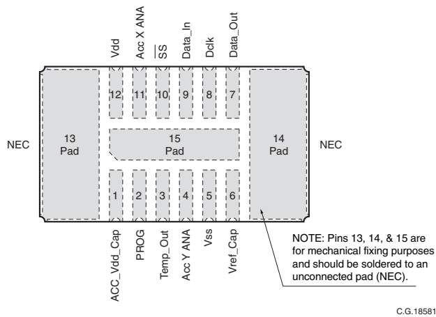
Figure 7.1 Pinout (Top View)
