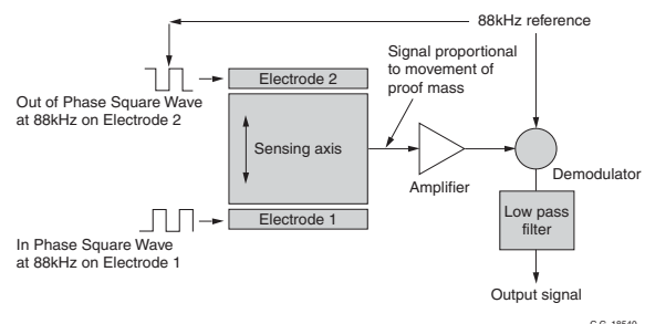
Figure 13.4(b) Schematic of Accelerometer Control Loop
