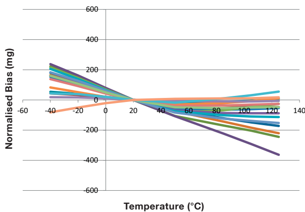
Figure 5.15: CAS215(96g) Accelerometer X Bias variation with Temperature
