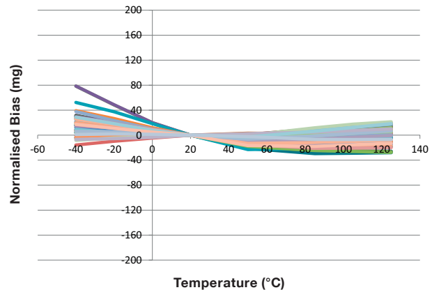
Figure 5.14: CAS214(30g) Accelerometer X Bias variation with Temperature
