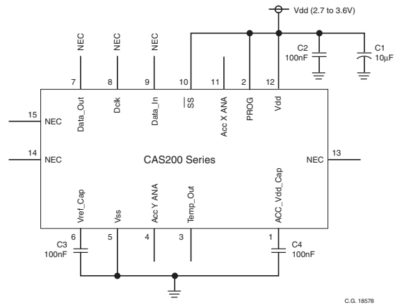
Figure 7.3 Analogue Output Setup
